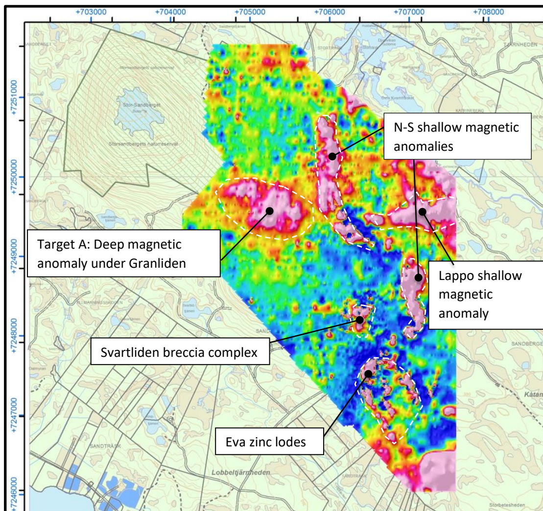
Figure 5: Map showing total magnetic field anomaly results.
