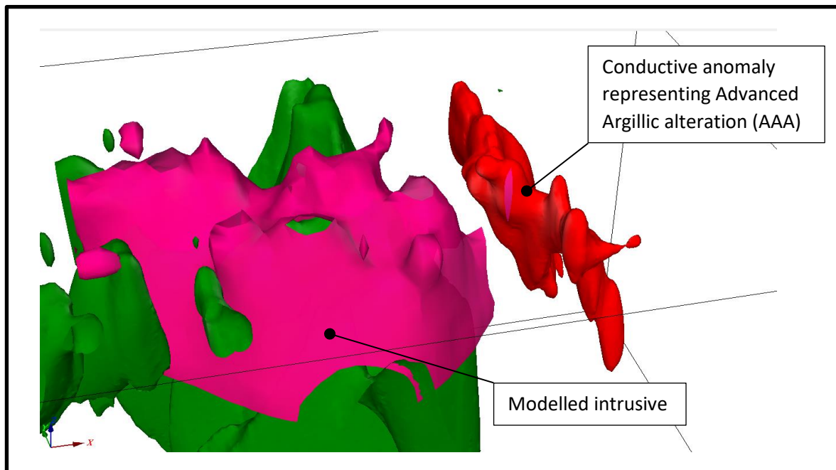
Figure 8: An interpreted intrusive feature modelled by NSAMT (in green) and by ground magnetics (in pink) is situated adjacent to the NSAMT AAA conductor (in red).
